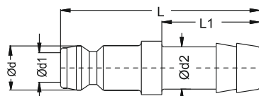
Standard Hose Plug Standard Schlauchtülle
