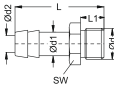
SHE nippel / SHE Nippel
